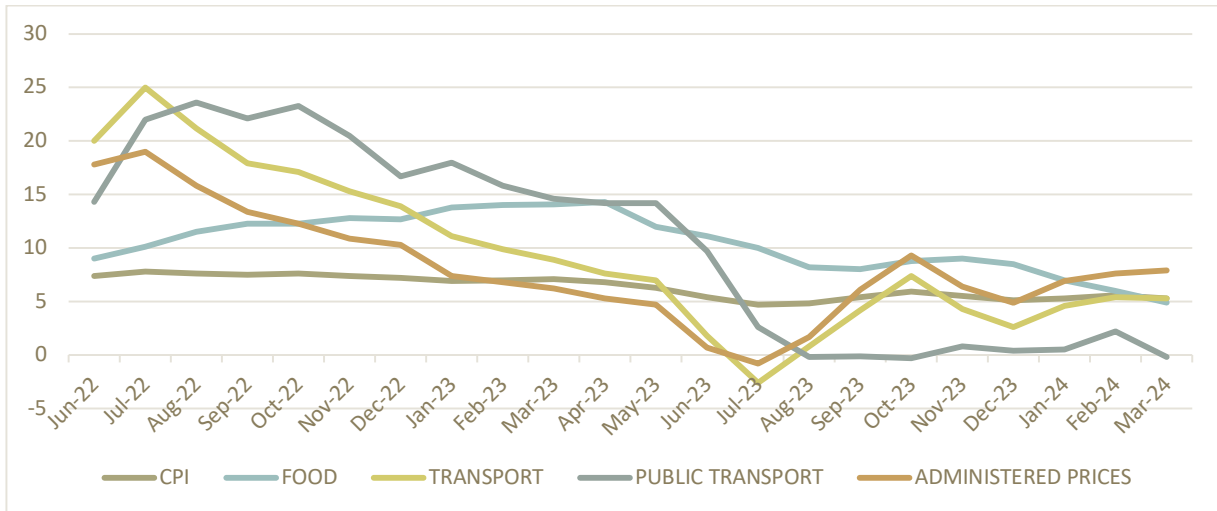
Figure 1: Consumer Price Index (CPI) and selected price categories | June 2022 to March 2024
