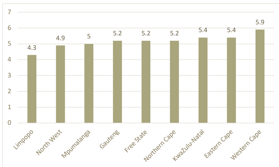
Figure 3: Annualised inflation rate (%) by province | March 2024
